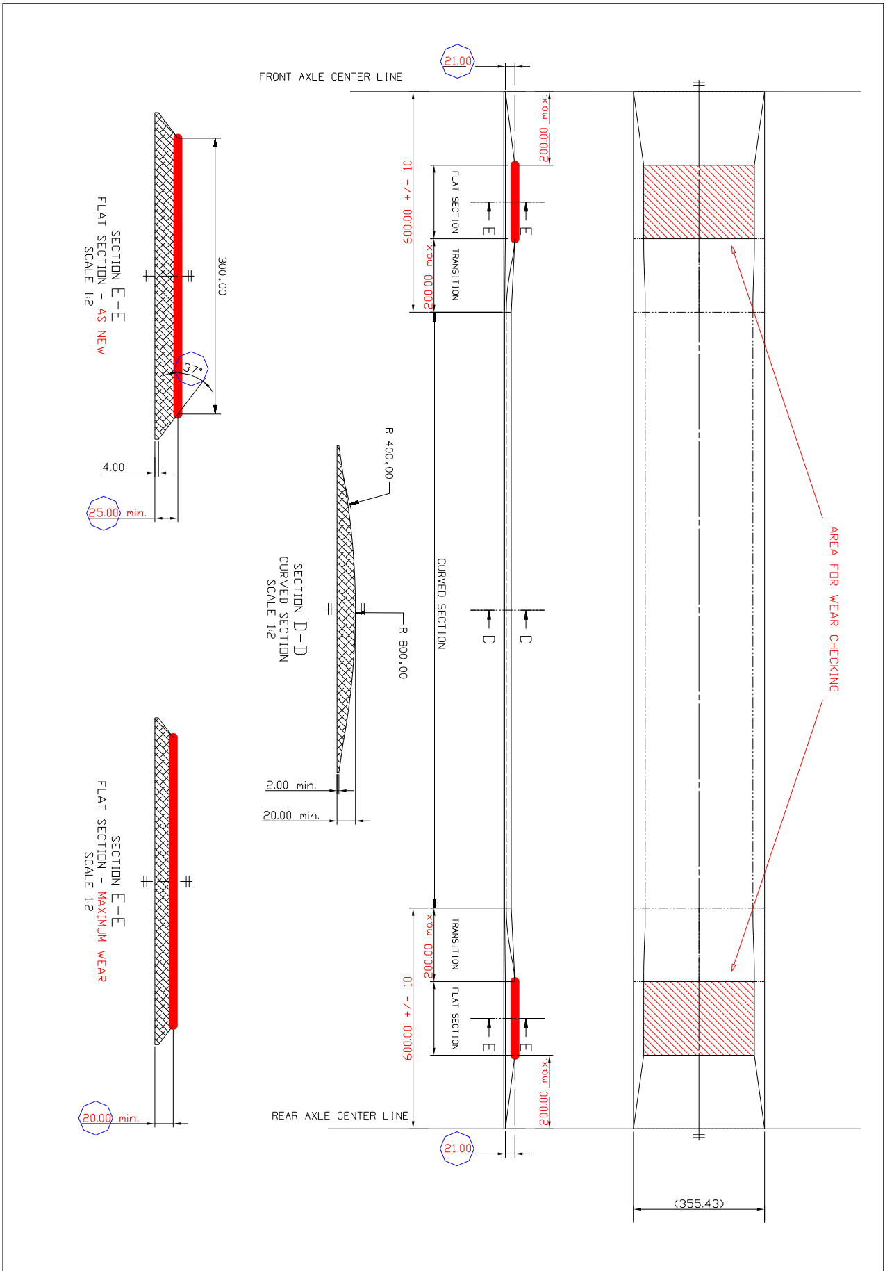
Dessin / Drawing 2
